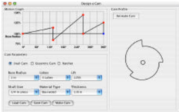
Figure 1. The MachineShop interface for creating a snail cam. In this scenario, we are creating a customized 3-lobed cam as described in the text.
