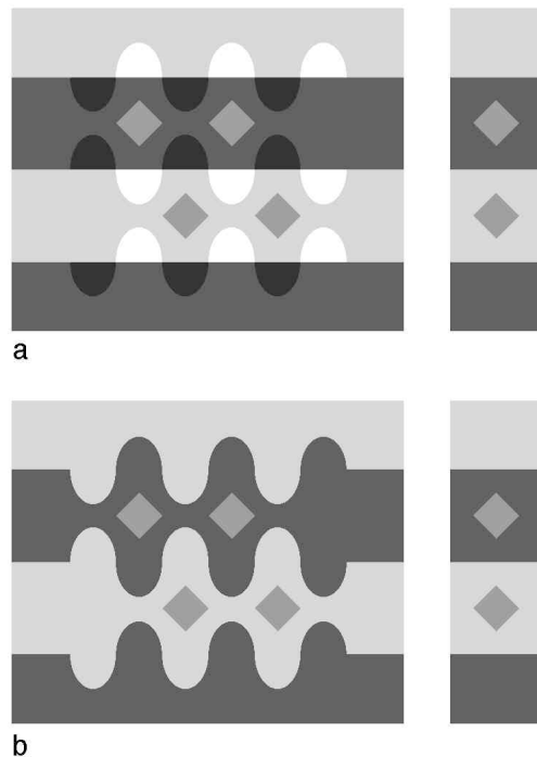
FIGURE 24.20 The snake illusion. All diamonds are the same shade of gray. (a) The regular snake: the diamonds appear quite different. (b) The "anti-snake": the diamonds appear nearly the same. The local contrast relations between diamonds and surrounds are the same in both (a) and (b).
